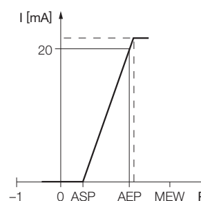
Fig. 10: Behavior of the current output (0...20 mA)
