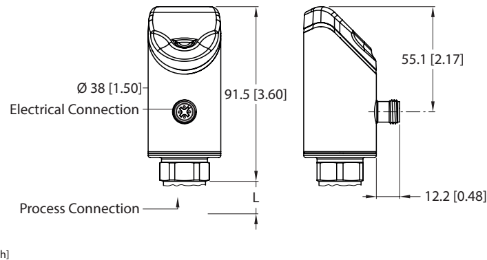
Fig. 2: Dimensions (mm)
